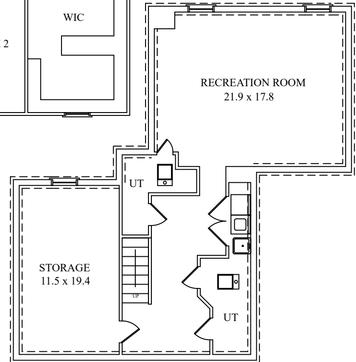
LOWER LEVEL
